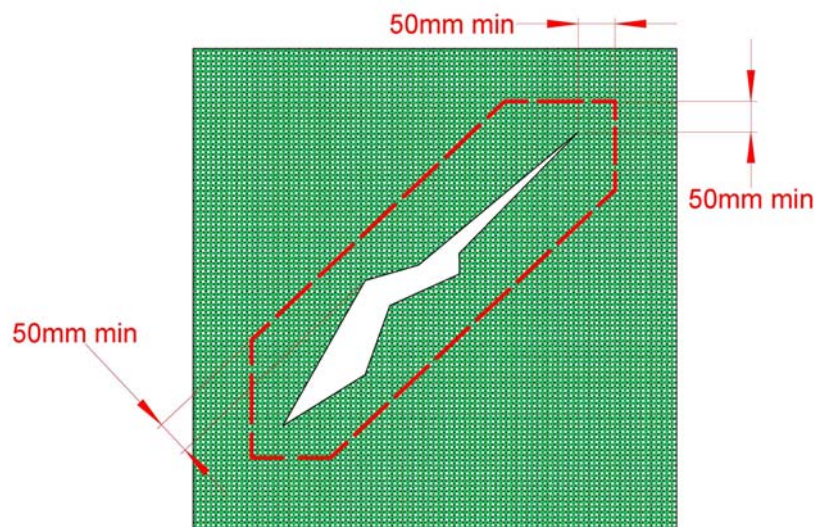
Figure 2, Cutting Repair Patch
