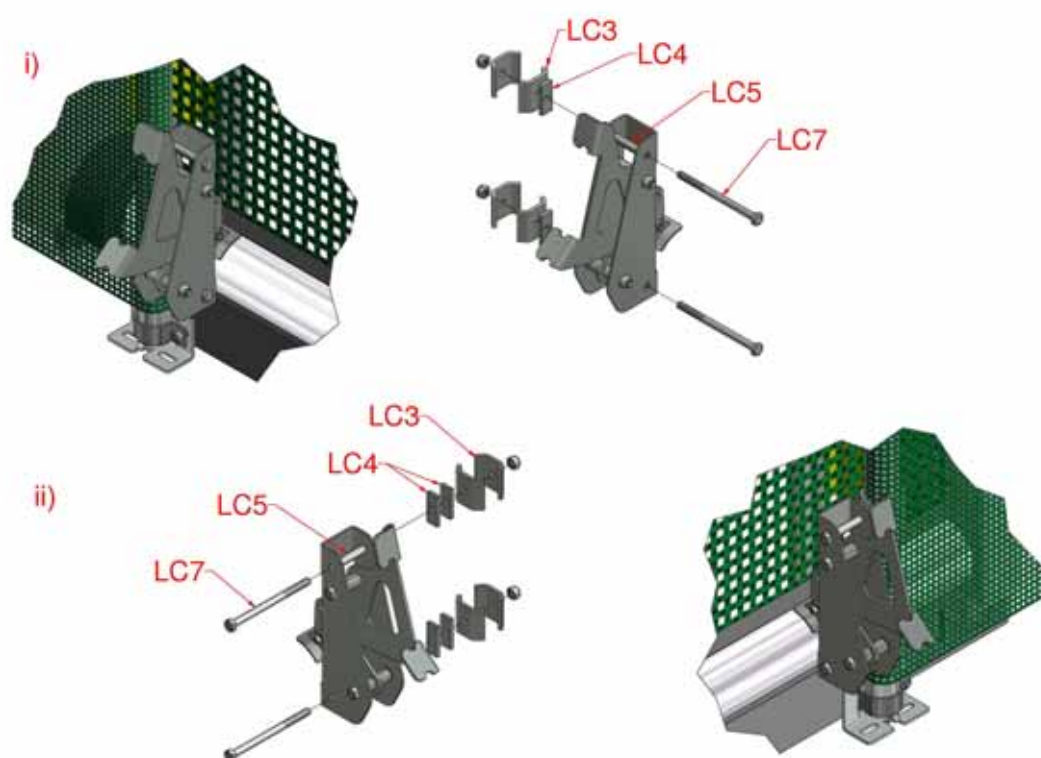
Figur 28, endelåsepaler
