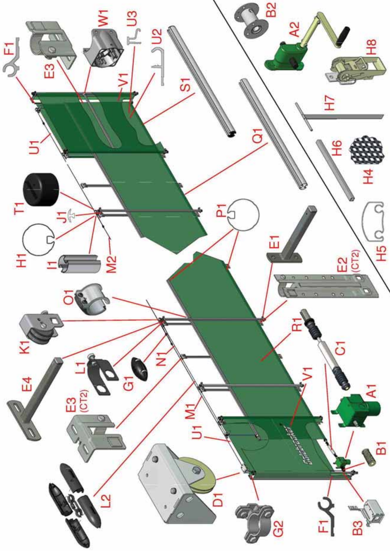
Figure 1a, System Overview (Bottom Rolling)
