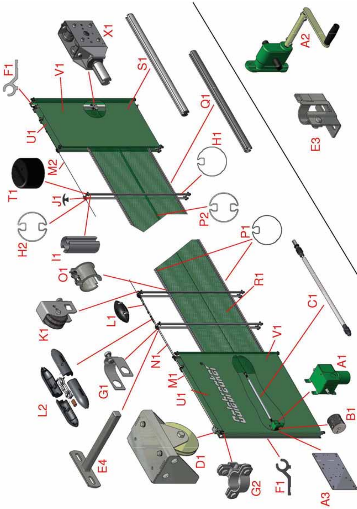
Figure 1b, System Overview (Middle Rolling)
