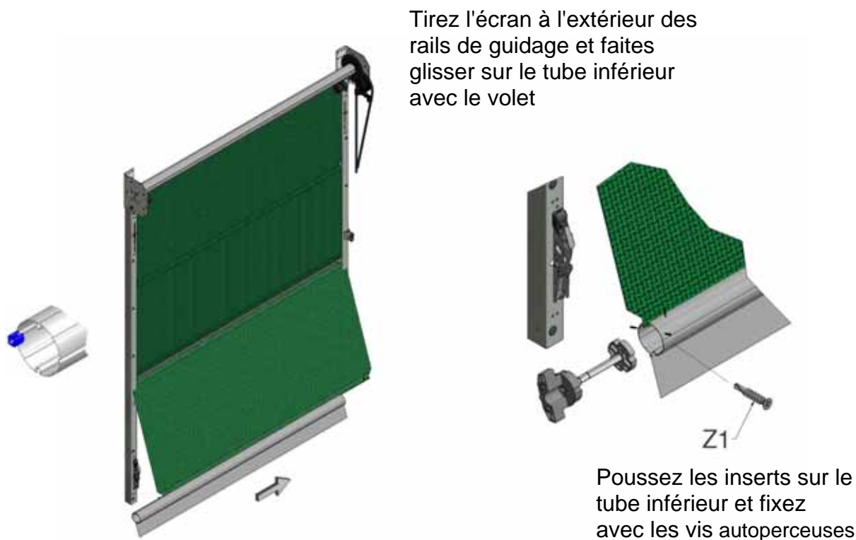
Figure 16a, attacher le tube inférieur
